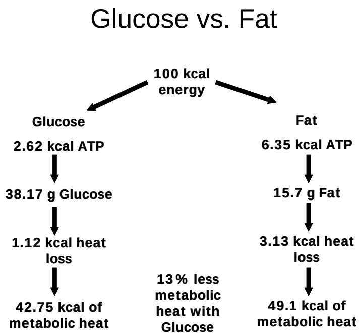
Figure 6. Bioenergetics and metabolic heat production from oxidizing either glucose or fatty acids (i.e. stearic acid) assuming 100 kcal of energy was needed and assuming 38 ATP/mole of glucose.
