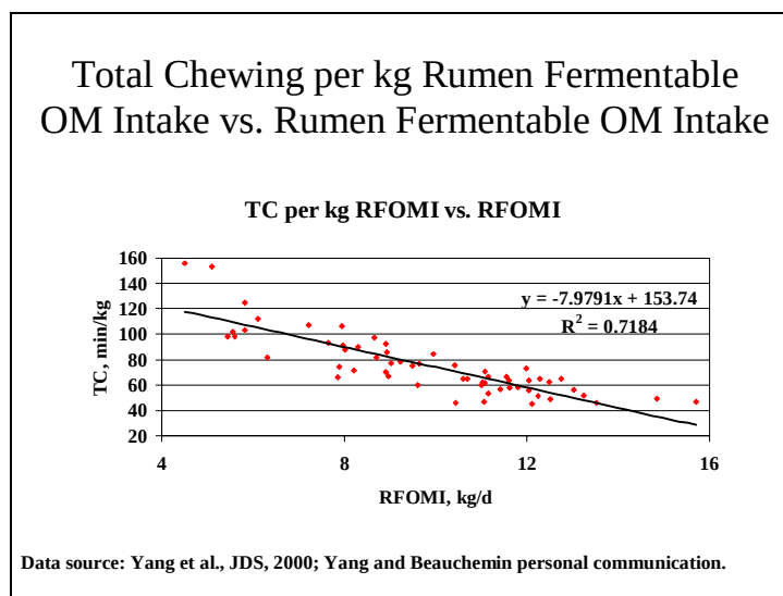
Figure 1. Relationship between total chewing time per kilogram of rumen-fermentable organic matter intake and intake of rumen fermentable organic matter.
