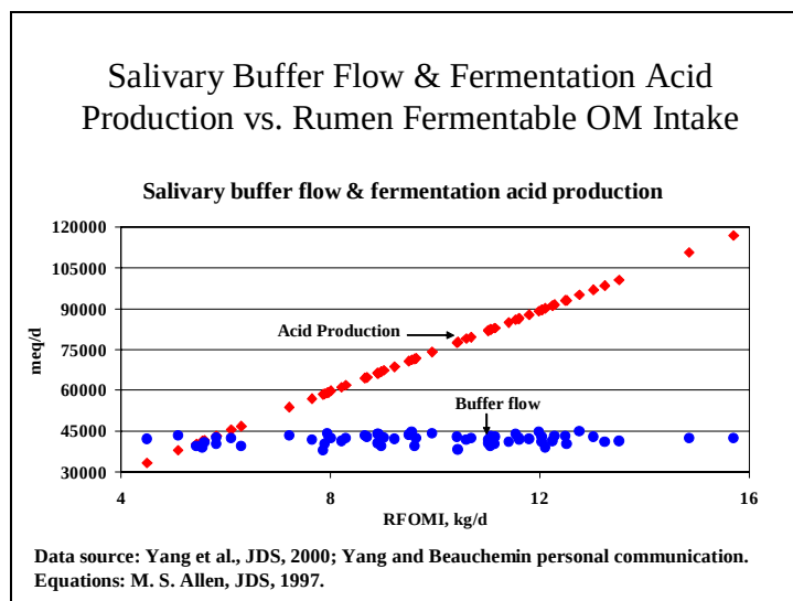
Figure 2. Calculated fermentation acid production and salivary buffer flow at varying intakes of rumen-fermentable organic matter.
